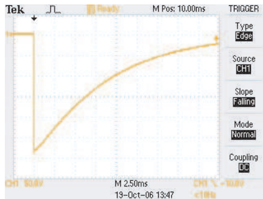
FIGURE 2. Voltage induced across the octupole magnet during a fast shutdown event. See text for details.
