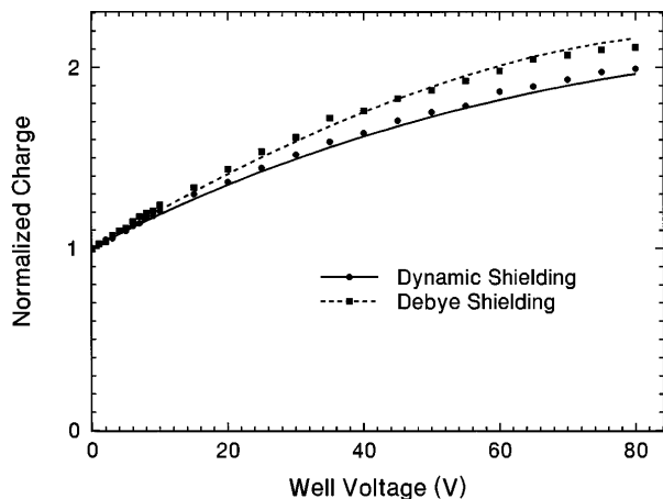
FIG. 6. Total charge vs well voltage. The “dynamic shielding” measurements were made immediately (1 ms) after the test well was adiabatically created, while the “Debye shielding” measurements were made after the plasma collisions were Maxwellian distributed, 1 s after the well was created. The lines are calculated from the theory described in the text.
