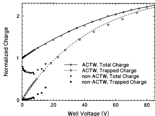
FIG. 4. Charge vs well voltage (depth). Measured values are indicated by the symbols, and the lines are calculated from the ACTW theory described in the text.
