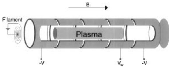
FIG. 2. Schematic of the experiment with a cutaway to show the plasma. Each cylinder is separately biasable.
