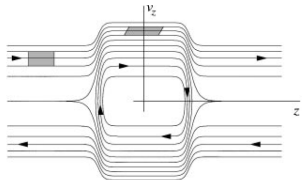
FIG. 1. Electron orbit phase space in the vicinity of a positive test well. Note the change in aspect of the square set of electrons as they propagate into the well.
