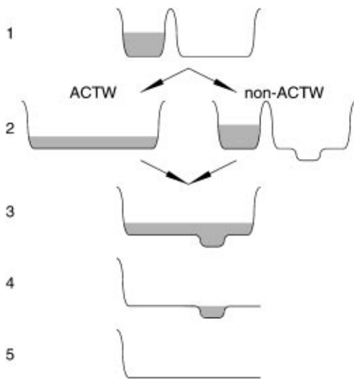
FIG. 3. Test well creation schemes. For clarity, the potentials are inverted. Step 1: Trap the initial plasma. Step 2: Adiabatic case (ACTW)—flood the plasma into the entire trapping region. Step 2: Nonadiabatic case (non-ACTW)—form the well. Step 3: ACTW—form the well and non-ACTW—flood the plasma into the entire trapping region. Step 4: Release and measure the image charge of the untrapped plasma. Step 5: Release and measure the image charge of the plasma trapped in the test well. The initial plasma length (step 1) is 12.8 cm, the final total plasma length is 29.3 cm, and the test well length is 11.5 cm.
