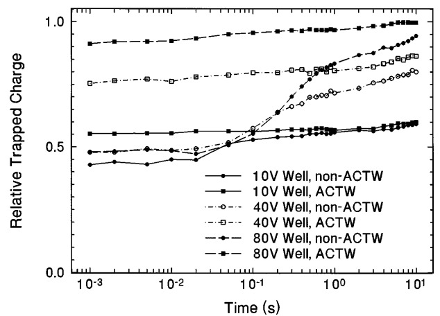
FIG. 5. Trapped charge normalized by total charge vs time for adiabatic and nonadiabatically created test wells, demonstrating the approach to equilibrium.
