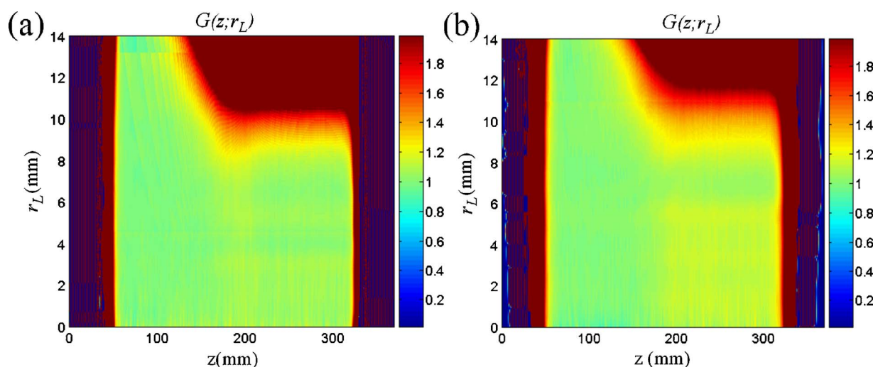
FIG. 12. (Color online). Color map of G(z; r_L) [defined in Eq. (2)] for (a) T=0.5 eV and (b) T=2.0 eV.
